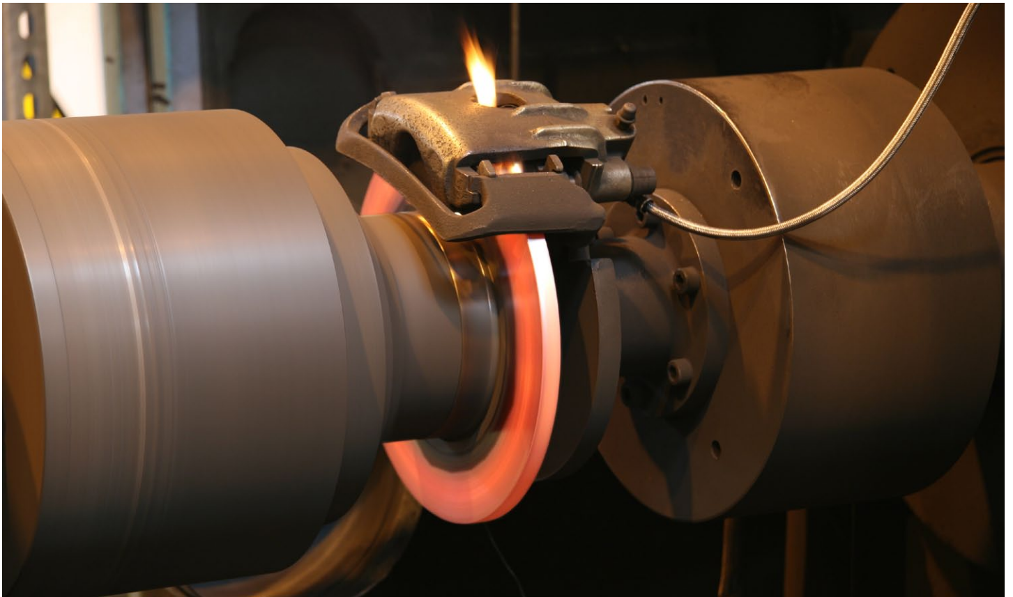
Dyno testing a Cosworth brake pad
